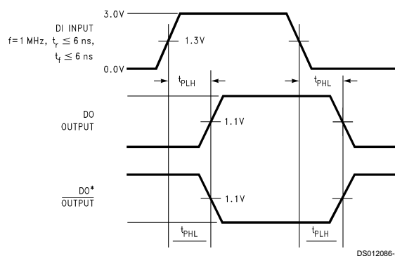
FIGURE 2. Propagation Delays
