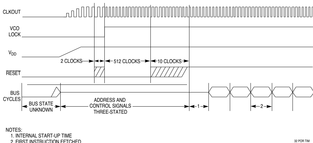
Figure 5-18 Power-On Reset
