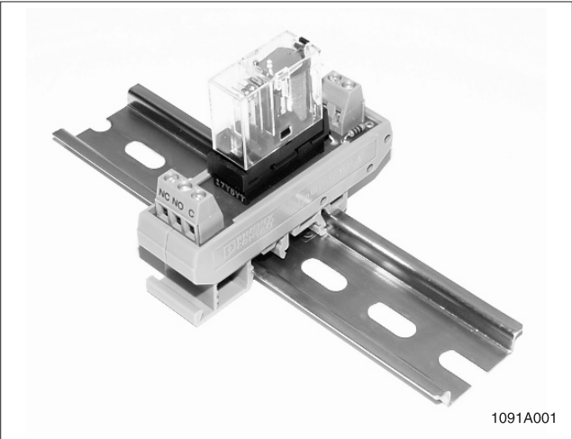
Figure 1. UMK 22-RELAY
