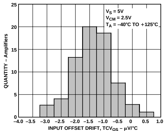
TPC 4. Input Offset Voltage Distribution ( TCV_{OS} )
