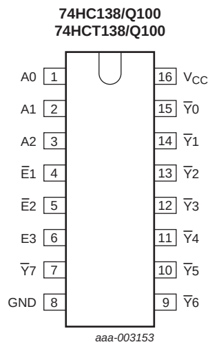
Fig 4. Pin configuration SO16 and TSSOP16
