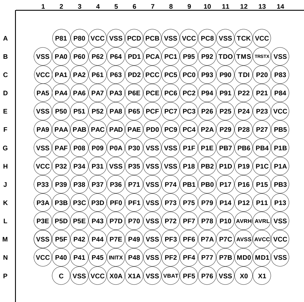
PFBGA-192
