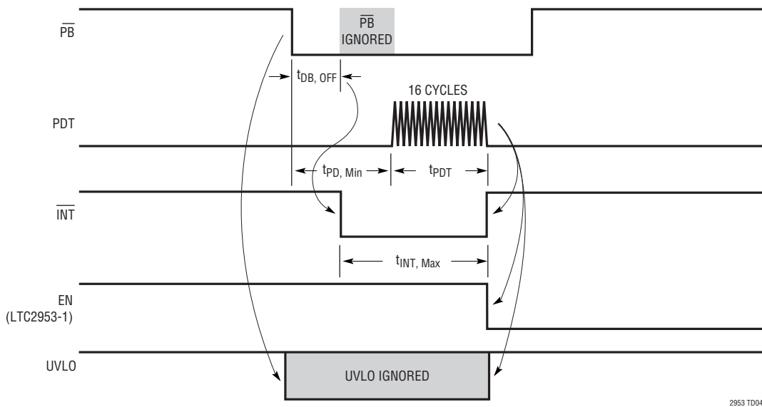
Figure 4. Push Button Power Down Timing: \overline{PB} Pressed and Held Low for t > (t_{PD, Min} + t_{PDT})
