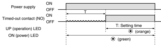
Time chart
