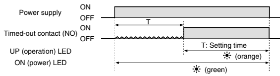
Time chart
