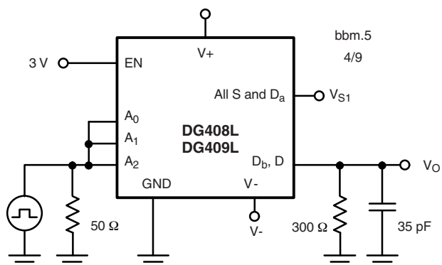
Figure 4. Break-Before-Make Interval
