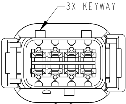
DTM04-08PD-E003 KEY -D- COLOR: BROWN
