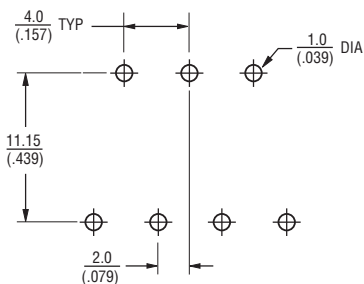
RECOMMENDED PWB PCB HOLE PATTERN
