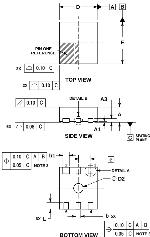
DFN6 2x2.2 mm CASE 488 ISSUE G
