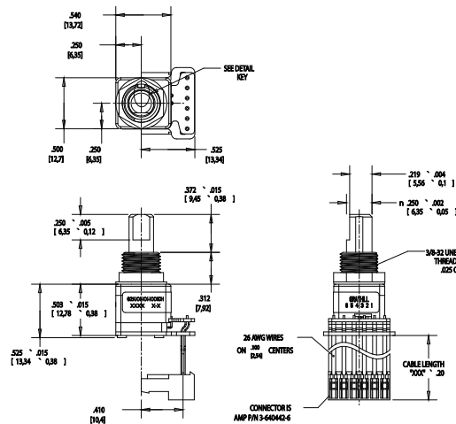
CH - CONNECTOR, 0.100" CENTERS
