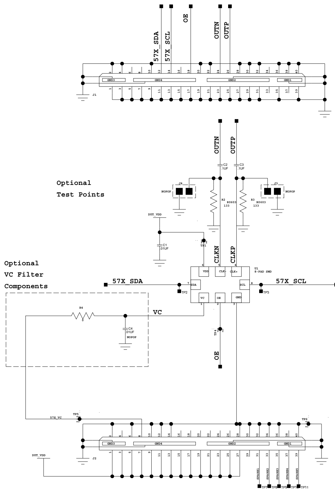
Figure 11. Si57x-EVB Daughterboard Schematic
