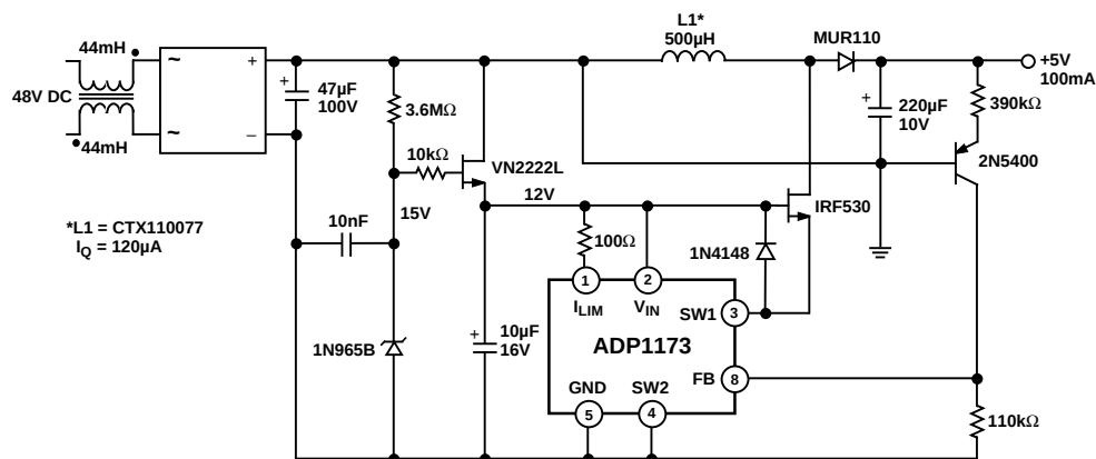
Figure 29. Telecom Supply
