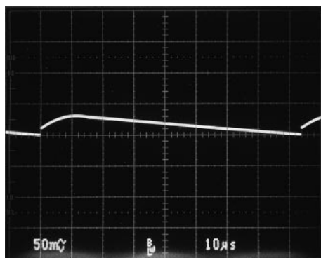
Figure 13. OS-CON Capacitor
