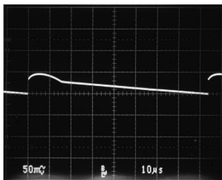
Figure 12. Tantalum Electrolytic
