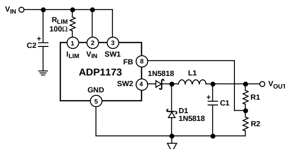
Figure 16. Step-Down Mode, V_{OUT} > 6.2 \text{ V}
