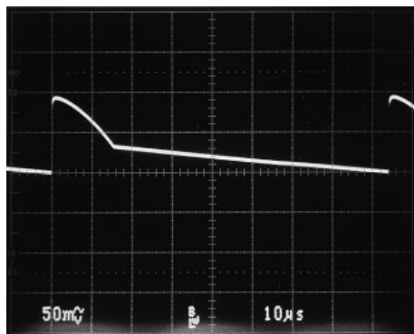
Figure 11. Aluminum Electrolytic
