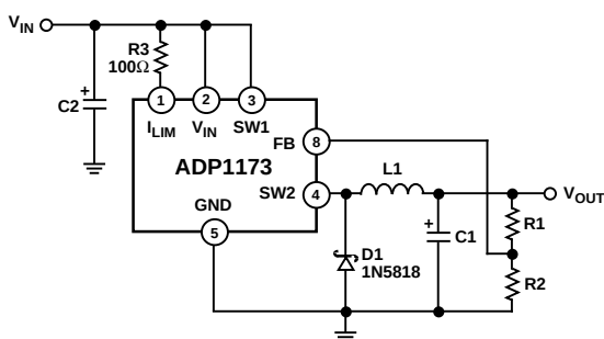
Figure 15. Step-Down Mode Operation
