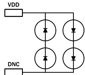
ESD CIRCUIT 3
