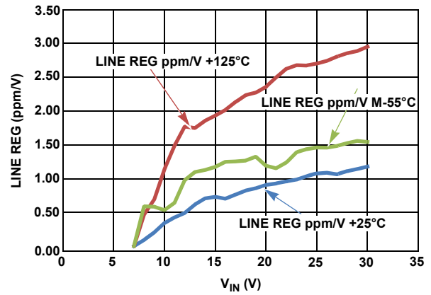
FIGURE 4. LINE REGULATION OVER TEMPERATURE
