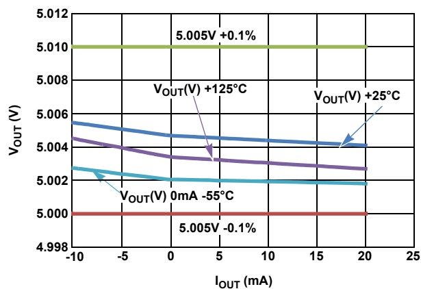
FIGURE 6. LOAD REGULATION OVER TEMPERATURE AT V_{IN} = 7V (V)
