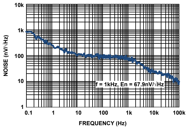
FIGURE 10. NOISE DENSITY vs FREQUENCY ( V_{IN} = 7.1V , I_{OUT} = 0mA , C_{IN} = 0.1\mu F , C_{OUT} = 1\mu F , COMP = 1nF )
