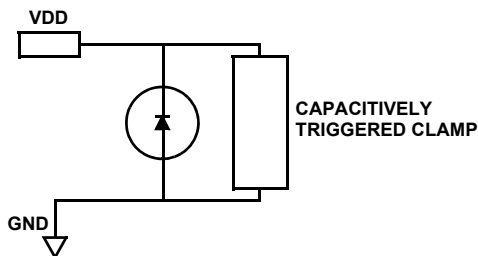
ESD CIRCUIT 1
