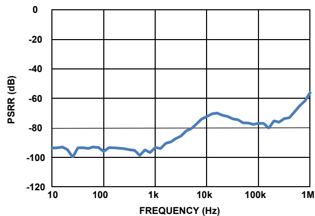
FIGURE 12. PSRR ( +25^\circ C , V_{IN} = 7V , V_{OUT} = 5.005V , I_{OUT} = 0mA , C_{IN} = 0.1\mu F , C_{OUT} = 1.0\mu F , COMP = 1nF , V_{SIG} = 300mV_{P-P} )
