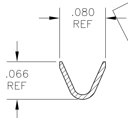
SECTION C-C
