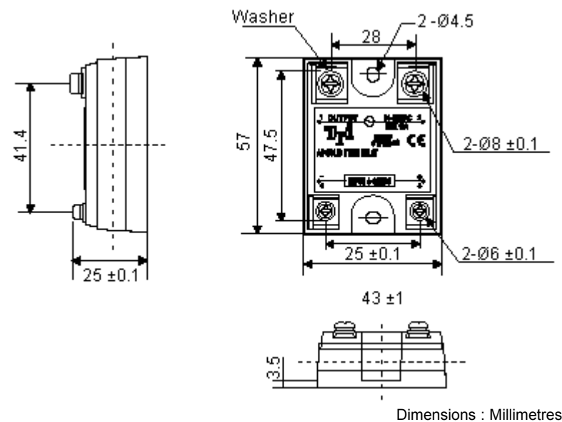
Outline Dimensions (Unit : mm)
