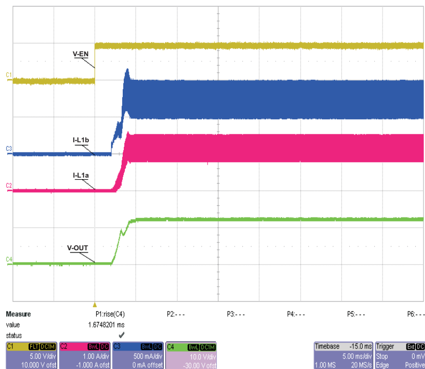
Figure 2. Start-Up With V_{IN} = 9\text{ V} and I_{OUT} = 750\text{ mA}
