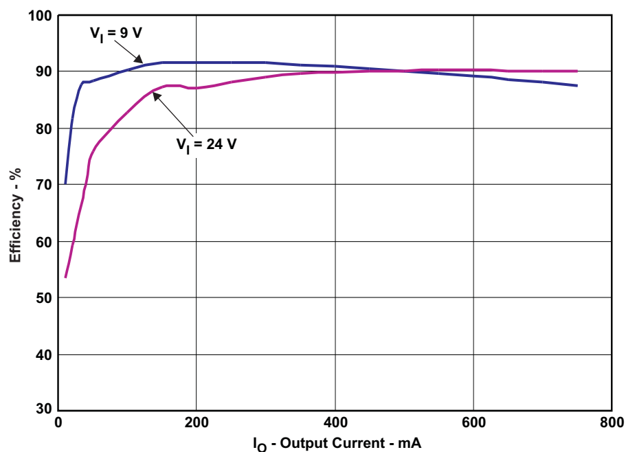
Figure 1. TPS61775EVM-588 Efficiency
