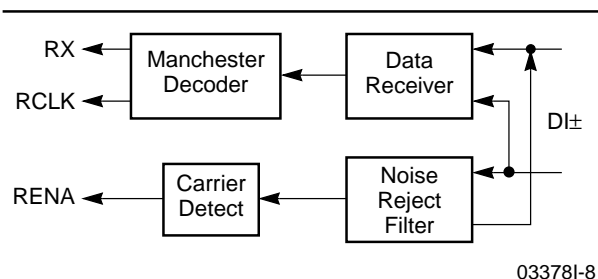
Figure 4. Receiver
