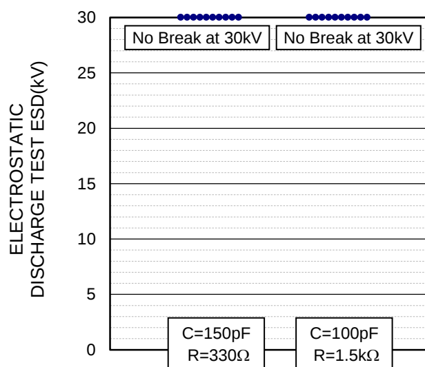
ESD DISPERSION
