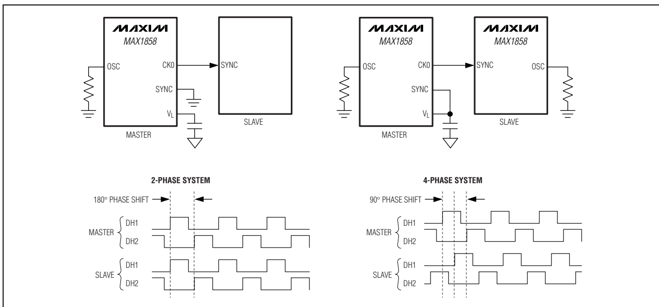
Figure 5. Synchronized Controllers
