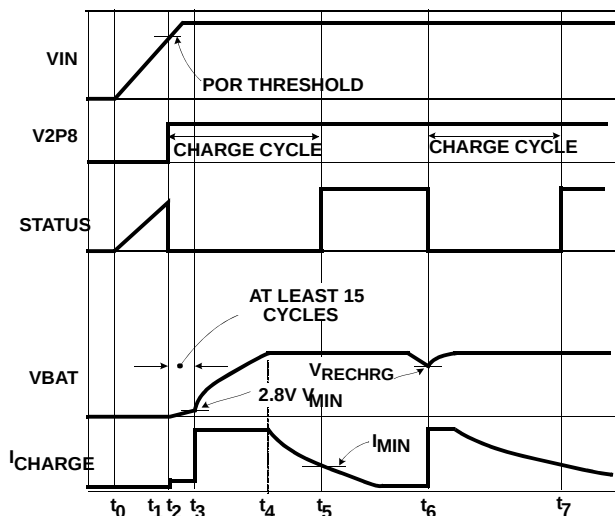
FIGURE 20. OPERATION WAVEFORMS
