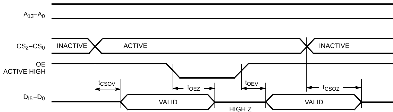
Chip Select and Output Enable Timing Diagrams
