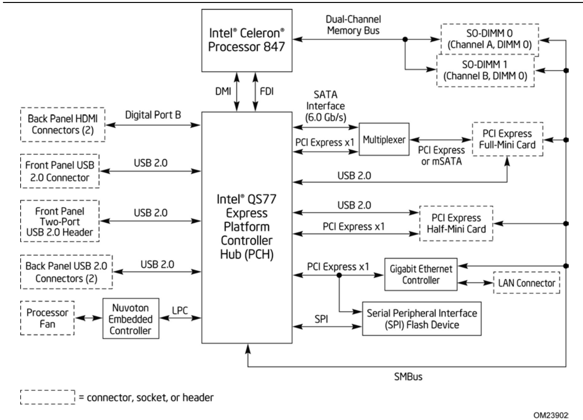
Figure 3. Block Diagram
