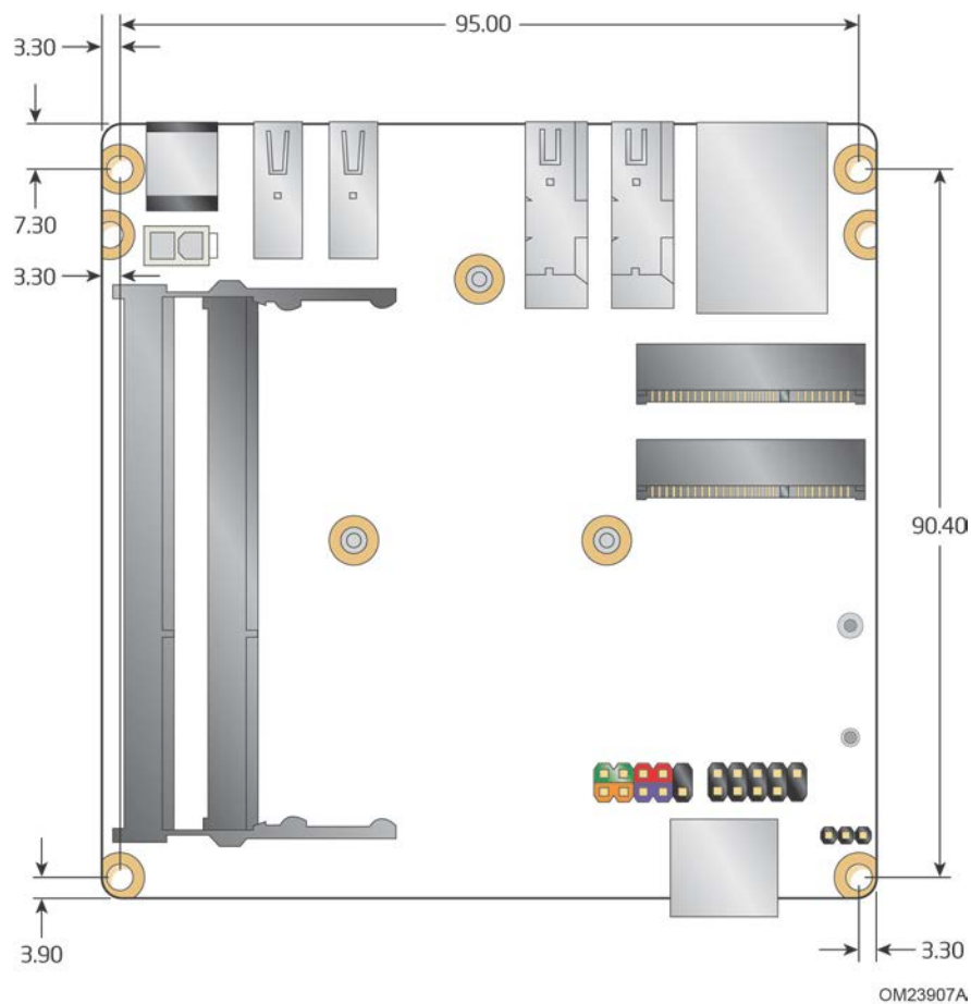
Figure 14. Board Dimensions
