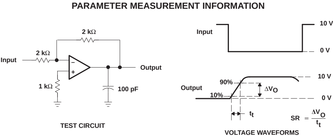
Figure 1. Slew Rate
