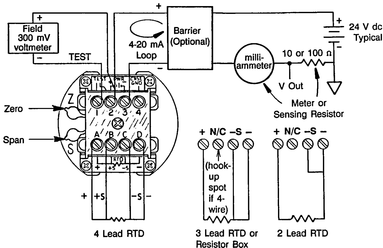
Figure 4-1 Input Connections
