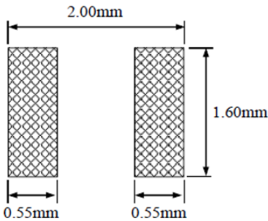
Dimension: mm
