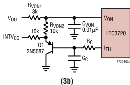
Figure 3. Correcting Frequency Shift with Load Current Changes
