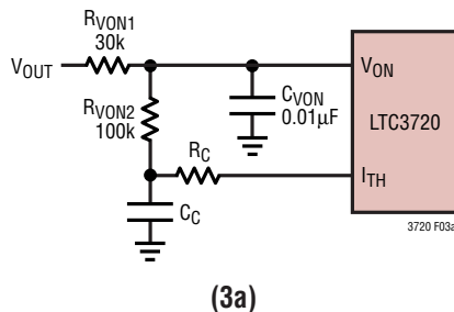
Figure 3. Correcting Frequency Shift with Load Current Changes
