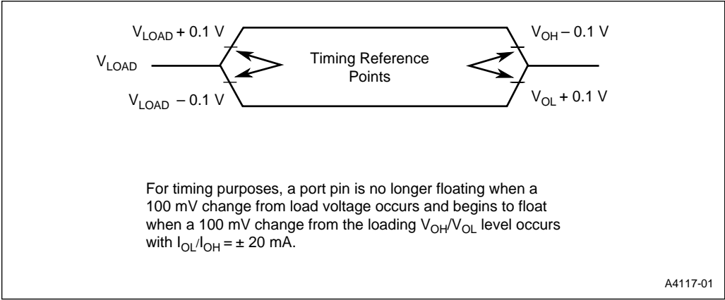
Figure 18. Float Waveforms
