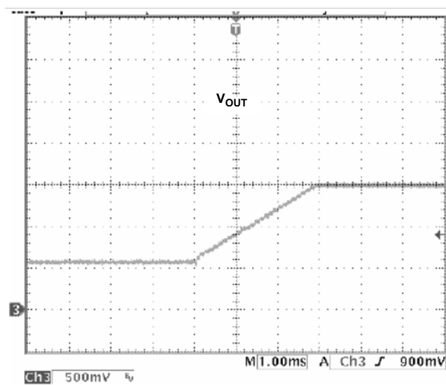
FIGURE 17. PRE-BIASED START-UP
