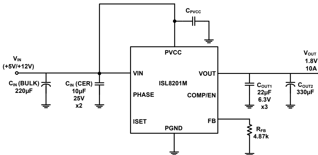
FIGURE 10. TYPICAL APPLICATION
