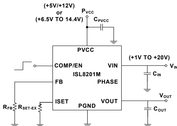
FIGURE 12. WIDE INPUT VOLTAGE APPLICATION SCHEMATIC
