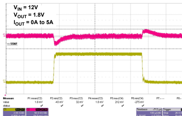
FIGURE 7. 1.8V TRANSIENT RESPONSE
