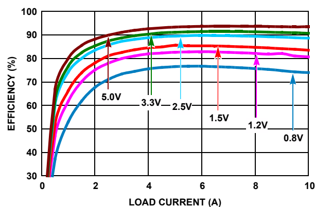
FIGURE 3. EFFICIENCY vs LOAD CURRENT ( 12V_{IN} )
