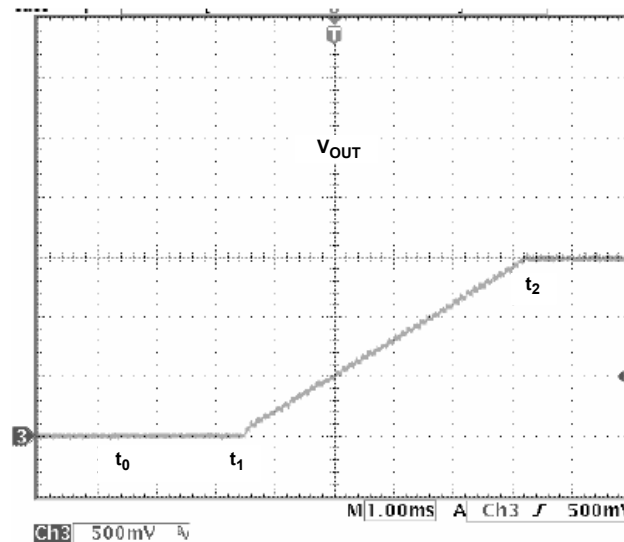
FIGURE 16. NORMAL START-UP
