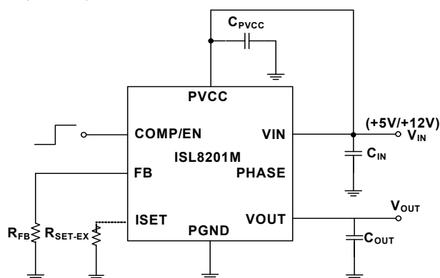
FIGURE 11. TYPICAL APPLICATION SCHEMATIC
