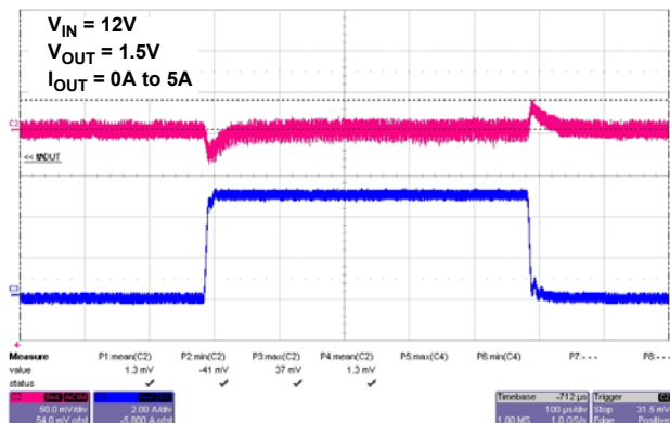
FIGURE 6. 1.5V TRANSIENT RESPONSE
