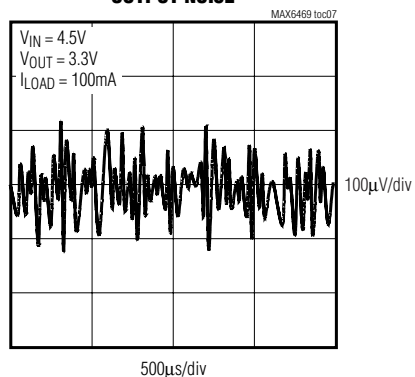
OUTPUT NOISE
