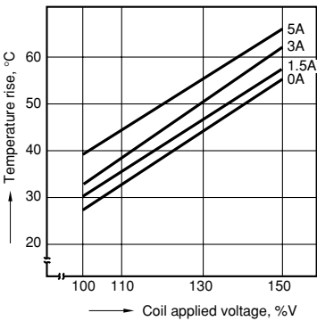
3. Coil temperature rise (at 30°C 86°F)
