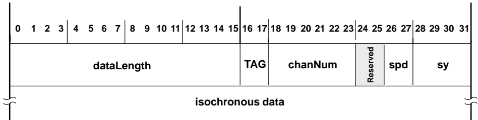
Figure 4–17. Isochronous-Transmit Format
