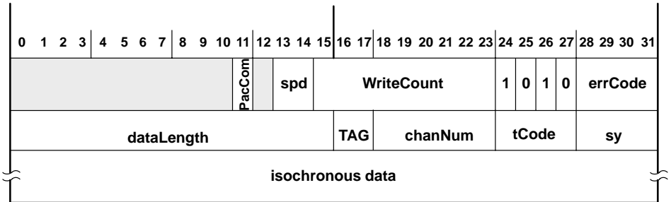
Figure 4–18. Isochronous-Receive Format
