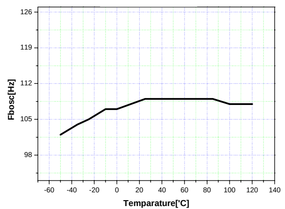
Figure 12. Operating Frequency
