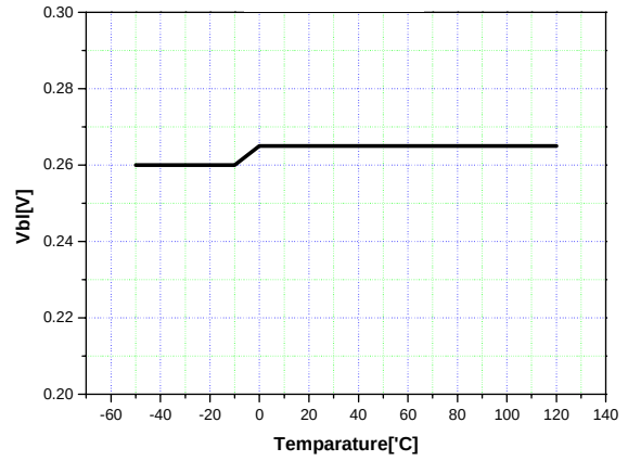
Figure 14. OSC Low Voltage
