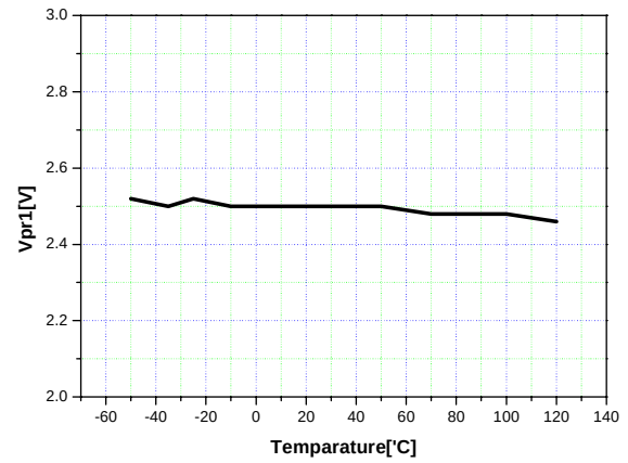
Figure 16. Open Lamp Protection Voltage 1
