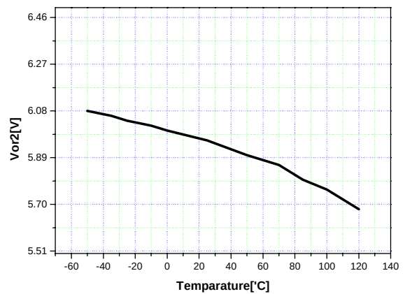
Figure 18. Open Lamp Regulation Voltage 2
