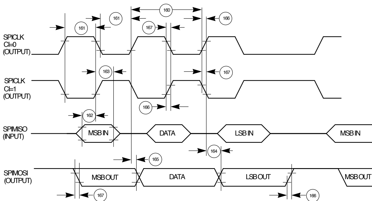
Figure 53. SPI Master (CP=1) Timing Diagram
