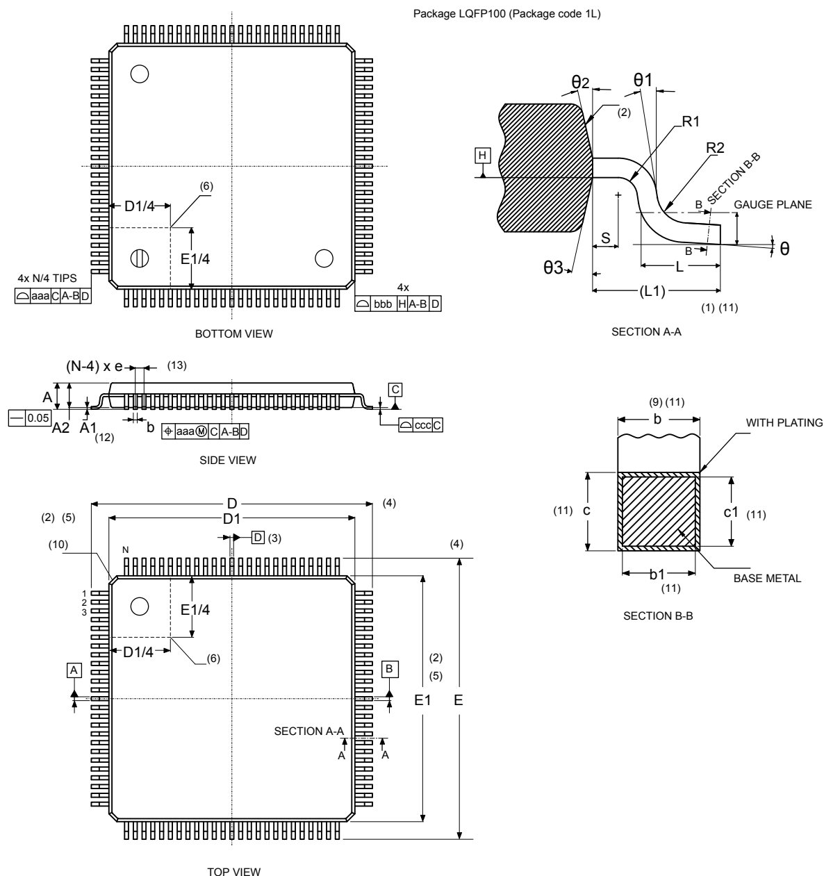
Figure 85. LQFP100 - Outline (15.)
