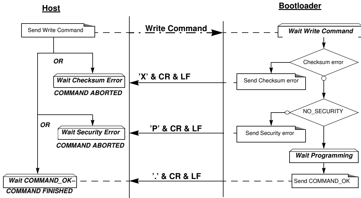
Figure 49. Write/Program Flow
