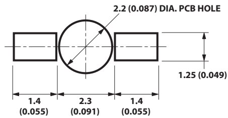
Figure 12. Recommended soldering pad pattern for HSMW-B265.
