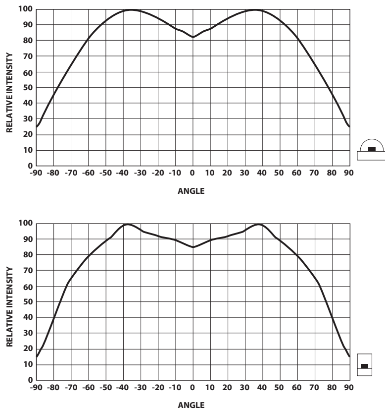
Figure 8. Relative intensity vs. angle for HSMW-B120.
