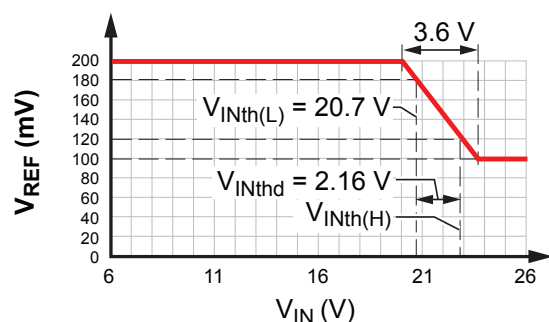
Figure 8: Output Current Foldback Based on V_{IN}
