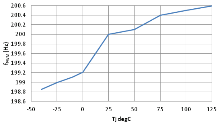
Figure 13: Temperature vs. f_{PWM} ( R_{FPWM} = 30.9 k \Omega )
