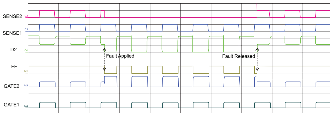
Figure 4B: Open-LED Fault on D2 with MODE = LOW and PWM Dimming
