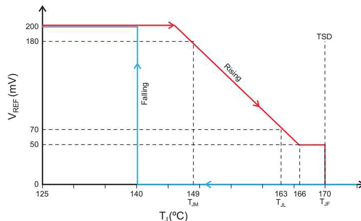
Figure 9: Output Current Foldback Based on Rising T_J
