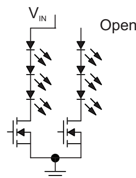
Figure 3: Open-LED Protection
