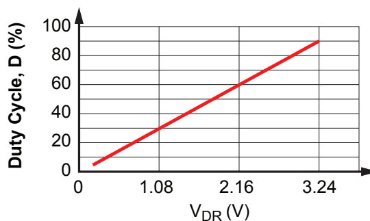
Figure 10: Relationship of External Voltage Input on DR Pin and Dimming Duty Cycle
