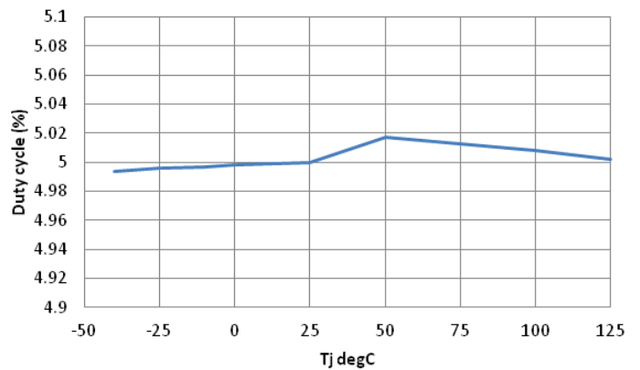
Figure 14: Temperature vs. Duty Cycle ( V_{VBIAS}/V_{DR} = 28.6 V/V)
