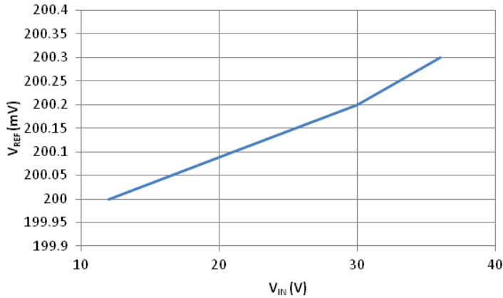
Figure 11: V_{IN} vs. V_{REF} ( V_{VTHTH} = 3.6 V)
