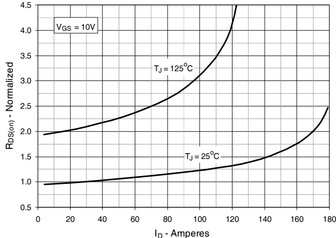
Fig. 5. R_{DS(on)} Normalized to I_D = 28A Value vs. Drain Current
