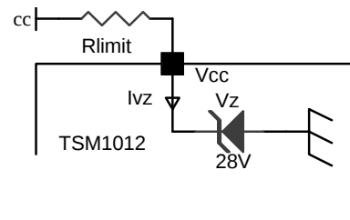
Figure 4 : Clamp voltage
