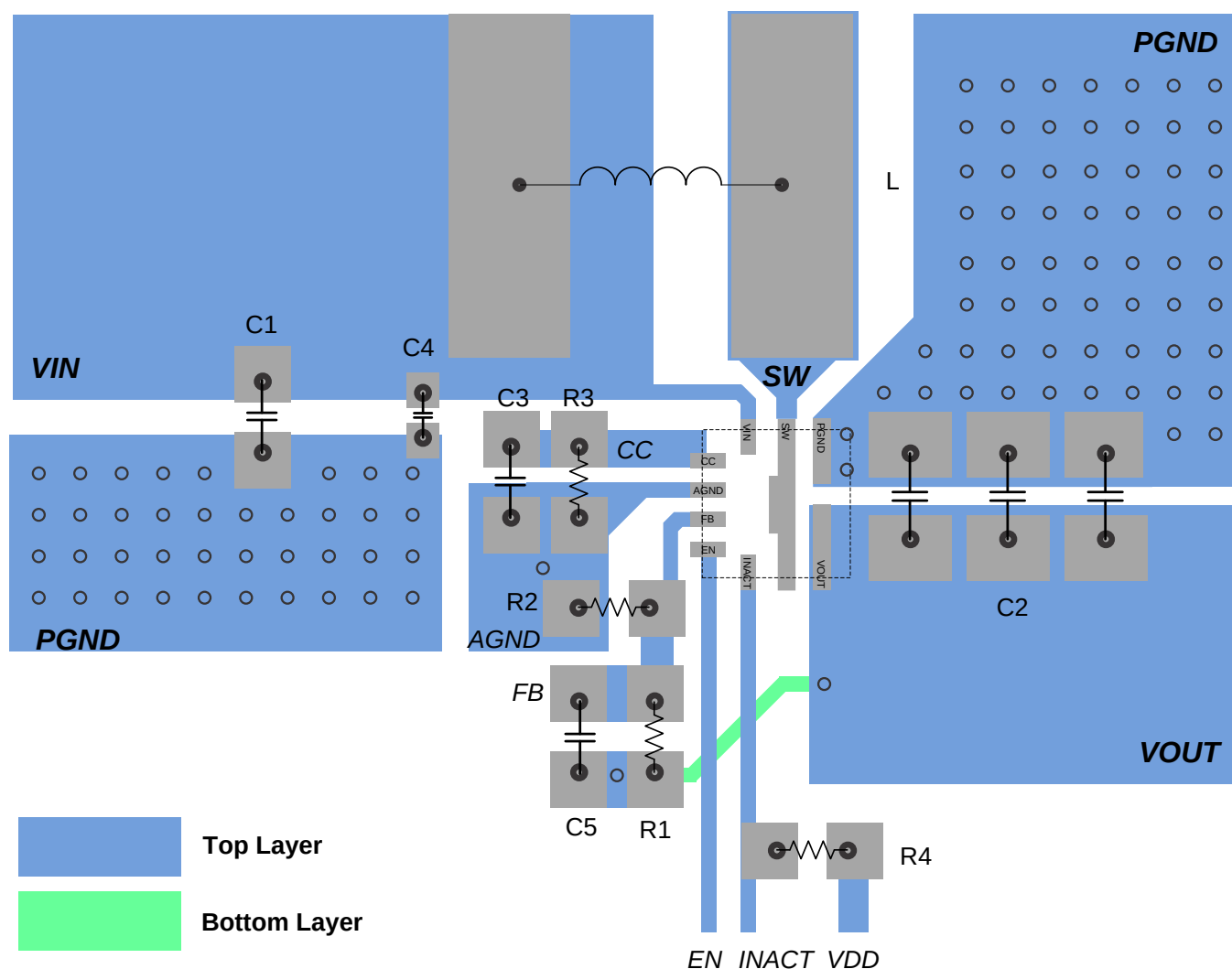
Figure 39. Layout Recommendation
