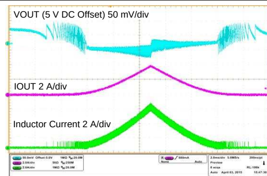
Figure 36. Load Regulation
