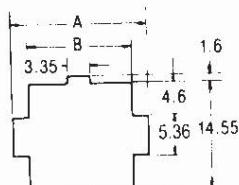
Cap Housing Panel Cutout
