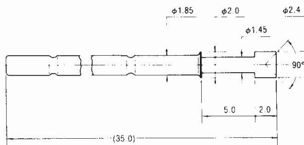
Part No. : 172971-1 (Phosphor Bronze/Nickel Plated)
