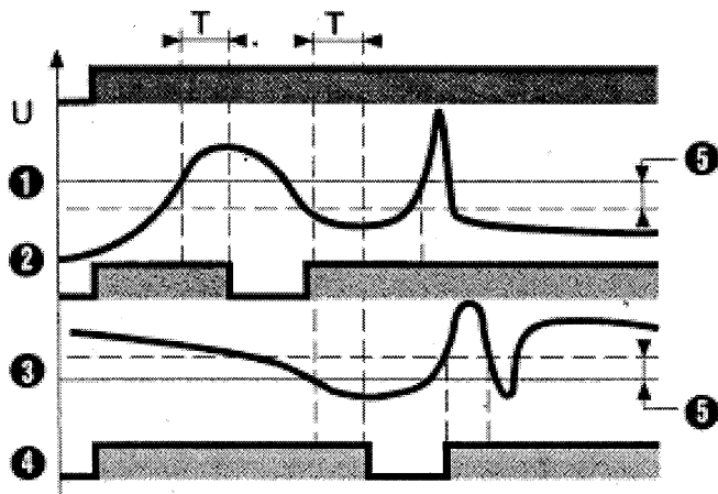
① Threshold ② Oper. R Overload ③ Threshold ④ Oper. R Underload ⑤ Hysteresis
