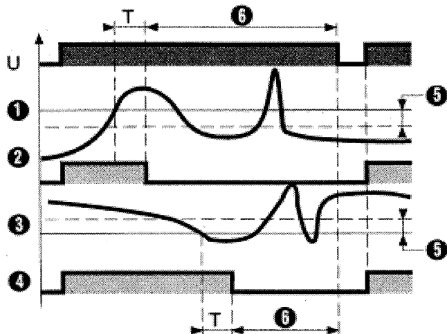
① Threshold ② Oper. R Overload ③ Threshold ④ Oper. R Underload ⑤ Hysteresis ⑥ Memory
