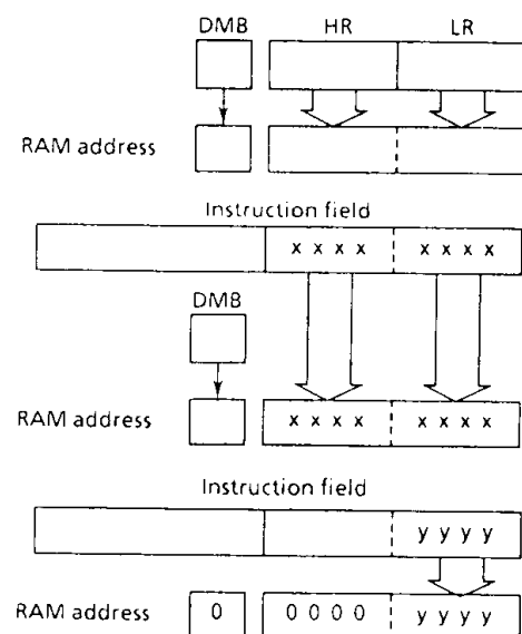
Figure 2-5. Addressing mode
