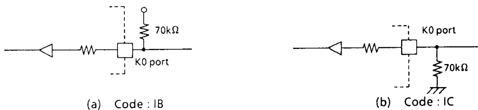
Figure 2. I/O code and external circuitry
