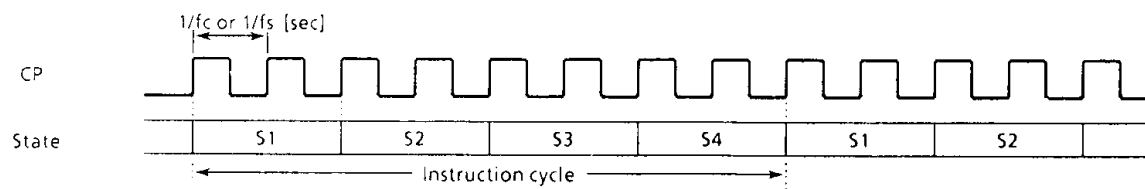
Figure 2-18. Instruction Cycle
