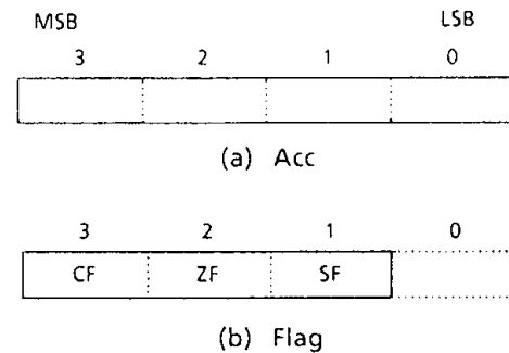
Figure 2-12. Acc, Flag
