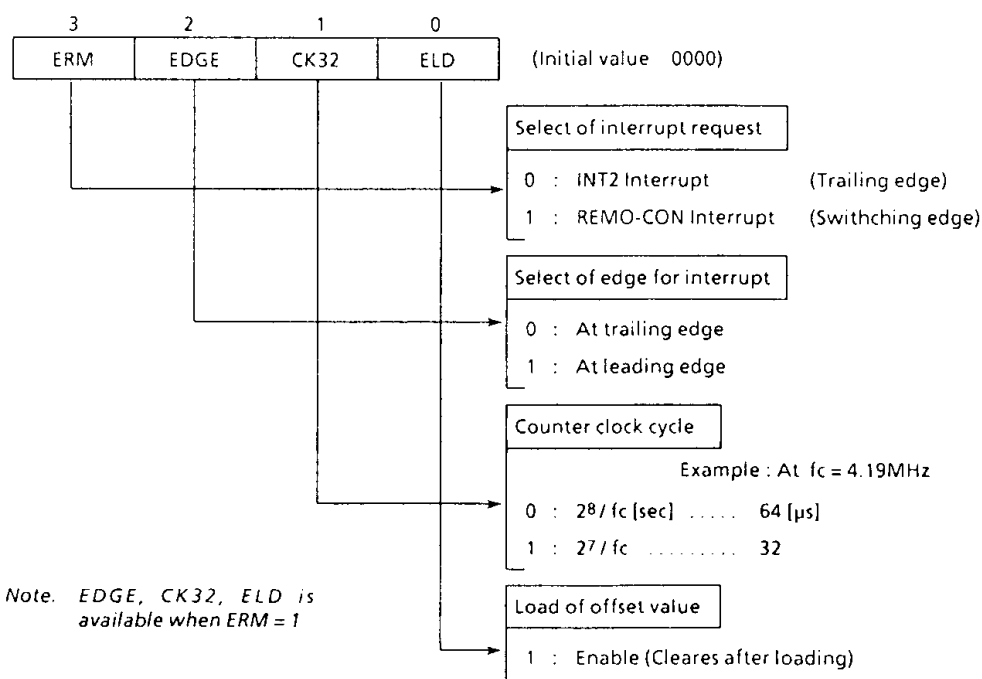
Figure 3-27. Command Register
