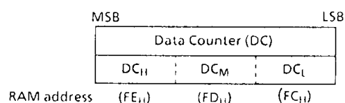
Figure 2-8. Data Counter
