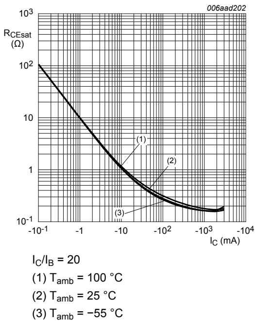
Fig. 24. TR2 (PNP): Collector-emitter saturation resistance as a function of collector current; typical values
