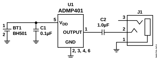
Figure 1. Evaluation Board Schematic
