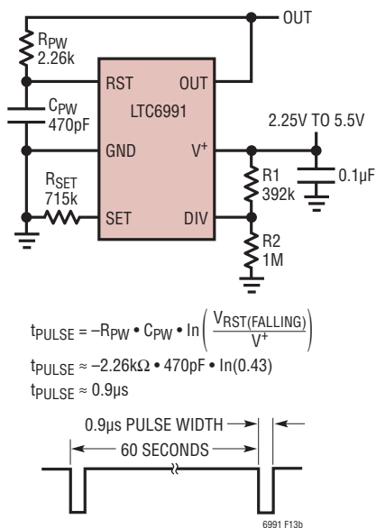
Figure 13b. Self-Resetting Circuit (DIVCODE = 11)
