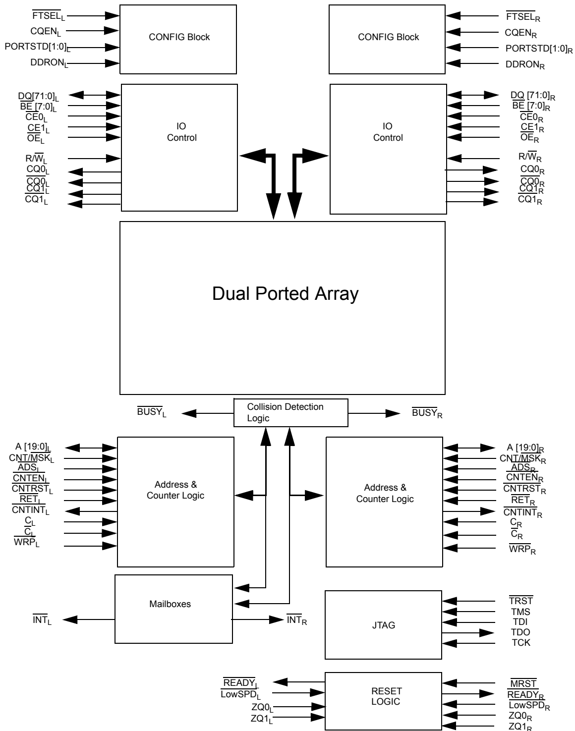
Figure 1. Block Diagram [1,2,3]
